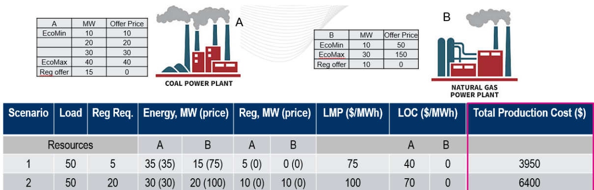
Figure 1: System Outcomes with Current Bidirectional Product
